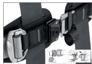
The FAST LT PIN-LOCK waistbelt buckle can only be unlocked with a special tool, limiting the risk of the participant opening the buckle.
