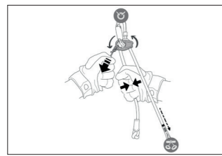
ADJUST features a hole for attaching a cord to more easily unblock the lanyard rope when it is weighted.
