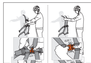
Easy to put on the participant, with FAST buckles at the rear of the harness.
