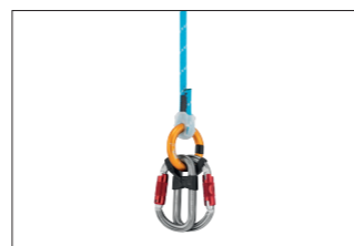
Termination with the STUART accessory, a RING OPEN gated ring, two Am'D TWIST-LOCK connectors equipped with CAPTIV positioning bars, allowing a climber to connect themselves.
